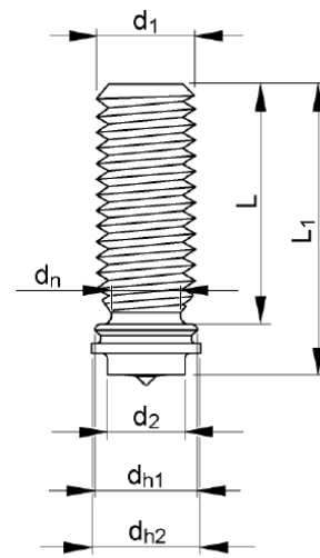
FIGURE 2B—F-BT-MR STUD
