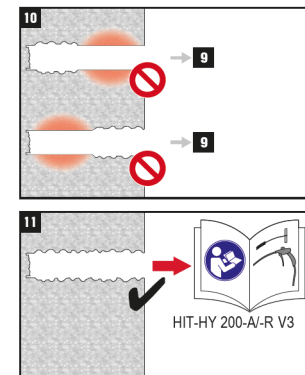
FIGURE 6—MANUFACTURER'S PRINTED INSTALLATION INSTRUCTIONS (MPII) (Continued)
